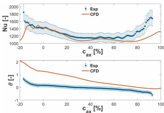
Figure 9. Lateral averaged Nusselt number (top) and adiabatic wall temperature (bottom) for CFD and experiments (IR 0.8%).
